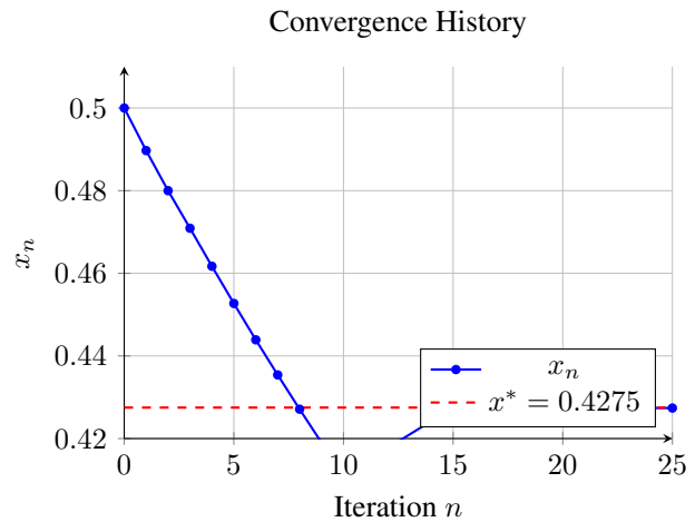
Figure 3. Iteration convergence to the fixed point
