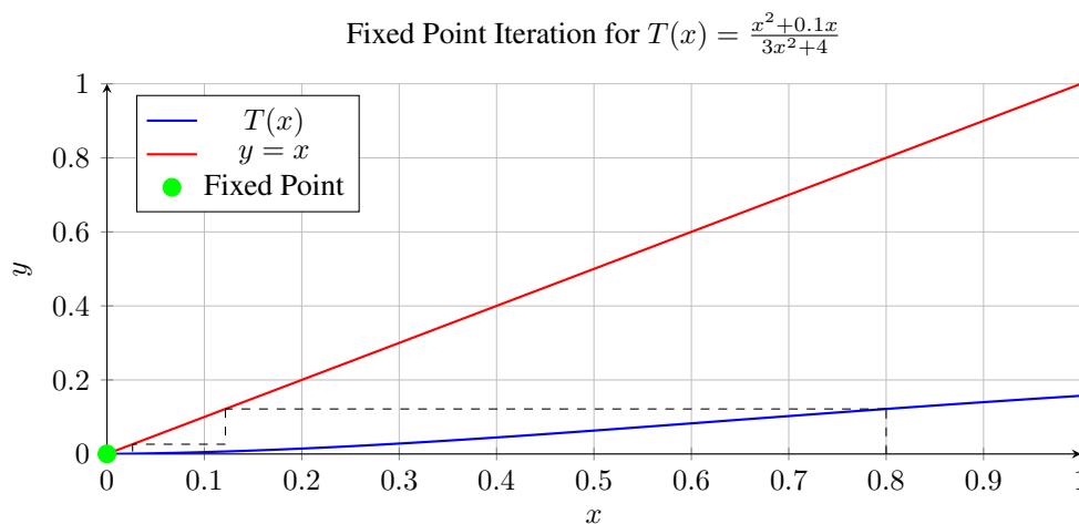
Figure 1. The convergence of iterations to the fixed point.
