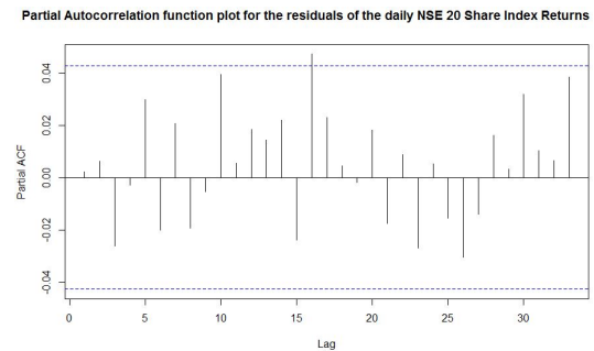
(a) ACF plot for the residuals of the daily NSE 20 share index return series. (b) PACF plot for the residuals of the daily NSE 20 share index return series.
