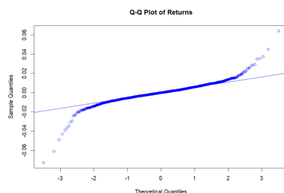
(c) QQ plot of the NSE 20 share index return series.
