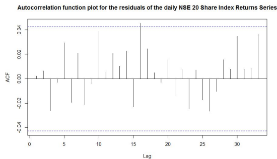
(a) ACF plot for the residuals of the daily NSE 20 share index return series. (b) PACF plot for the residuals of the daily NSE 20 share index return series.
