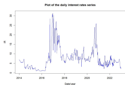
(a) plot of the interest rate series.
