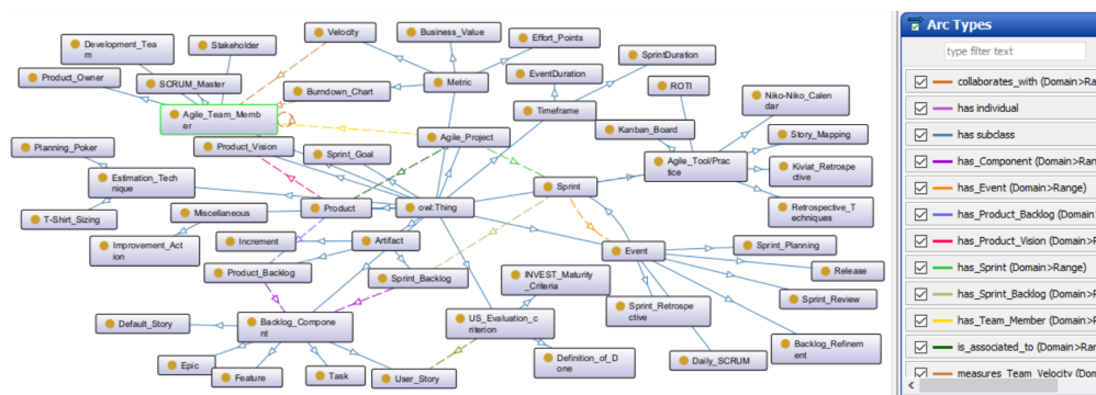
Figure 3. The proposed Agile Project Management Ontology developed in OWL using Protégé 5.
