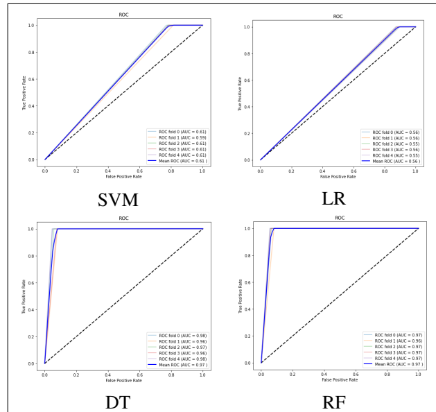
Figure 11. ROC Curve for dataset-1(with Feature Reduction)
