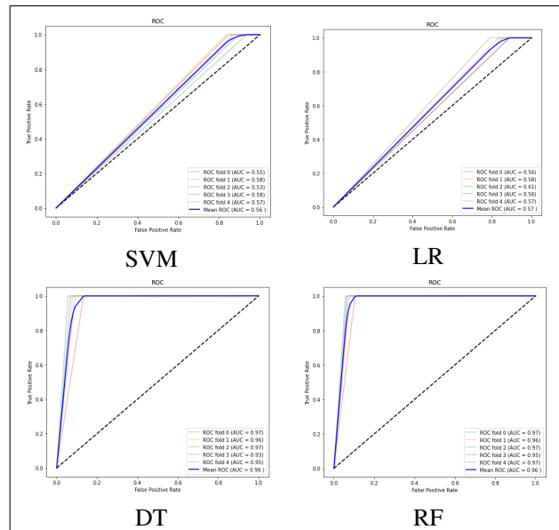
Figure 13. ROC Curve for dataset-2(with Feature Reduction)
