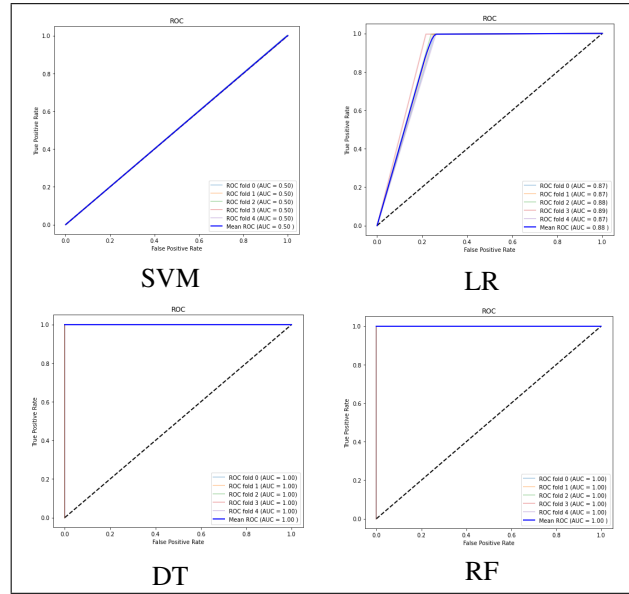
Figure 10. ROC Curve for dataset-1(without Feature Reduction)
