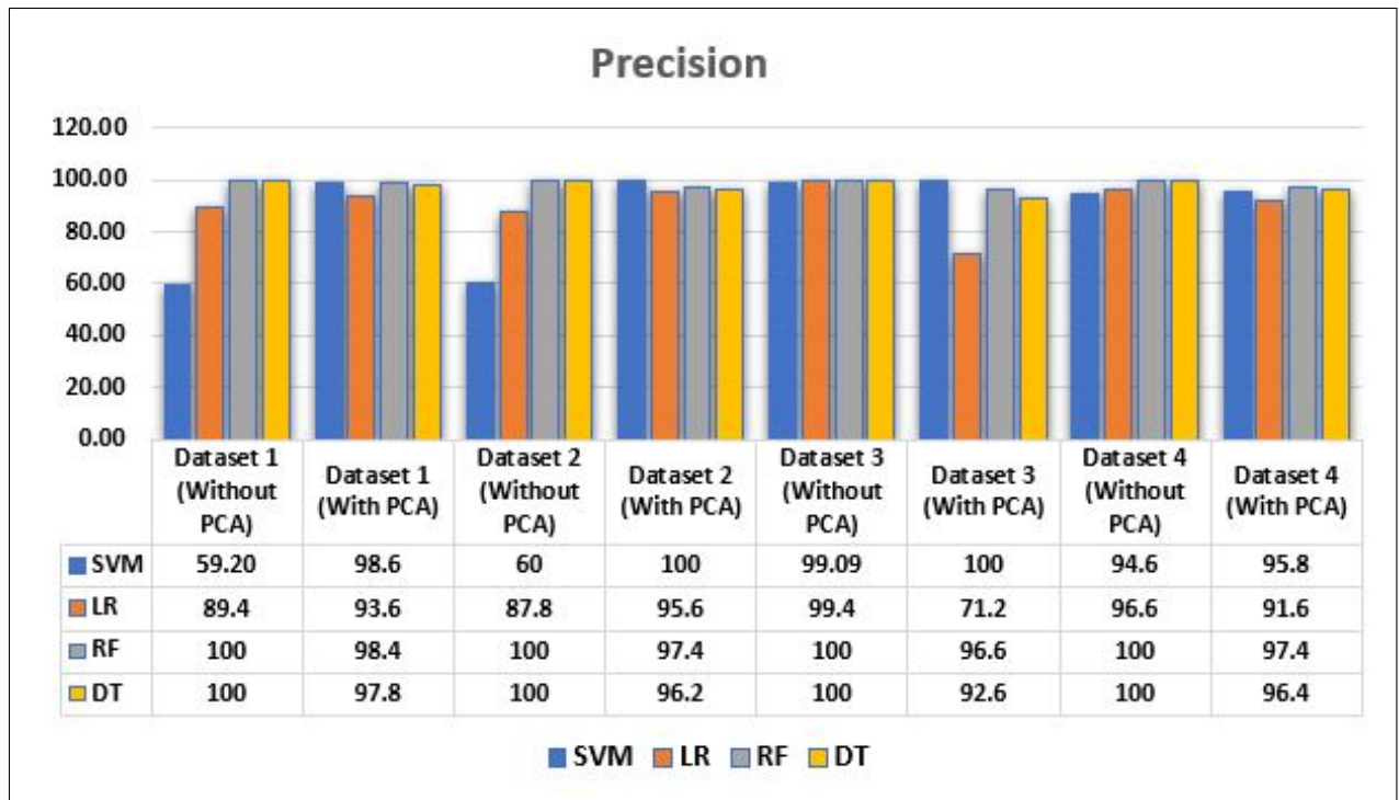
Figure 8. Precision result for all the Dataset
