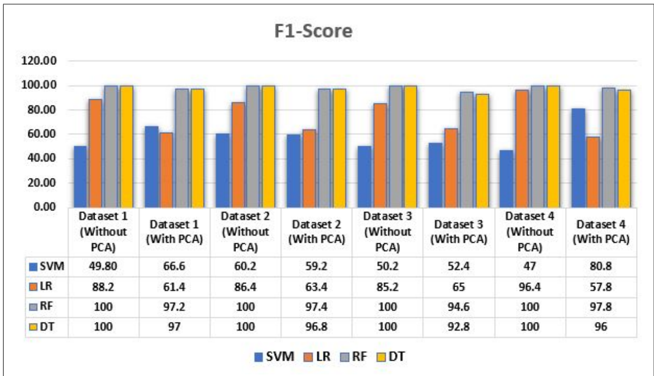
Figure 7. F1-Score result for all the Datasets
