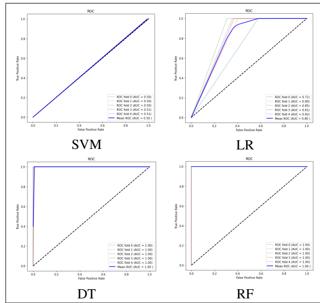
Figure 12. ROC Curve for dataset-2(without Feature Reduction)
