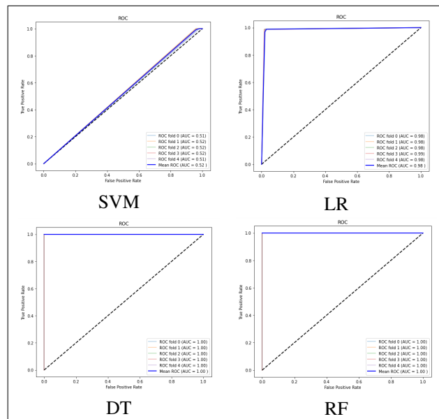
Figure 16. ROC Curve for dataset-4(without Feature Reduction)
