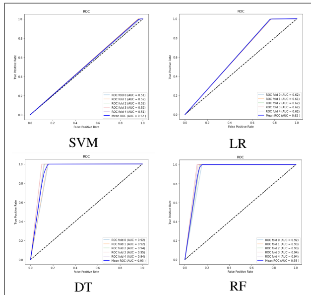
Figure 15. ROC Curve for dataset-3(with Feature Reduction)
