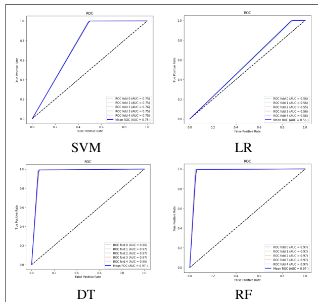
Figure 17. ROC Curve for dataset-4(with Feature Reduction)
