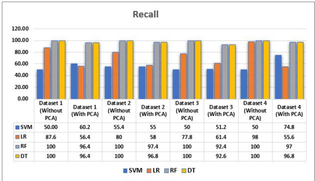
Figure 9. Recall result for all the Dataset
