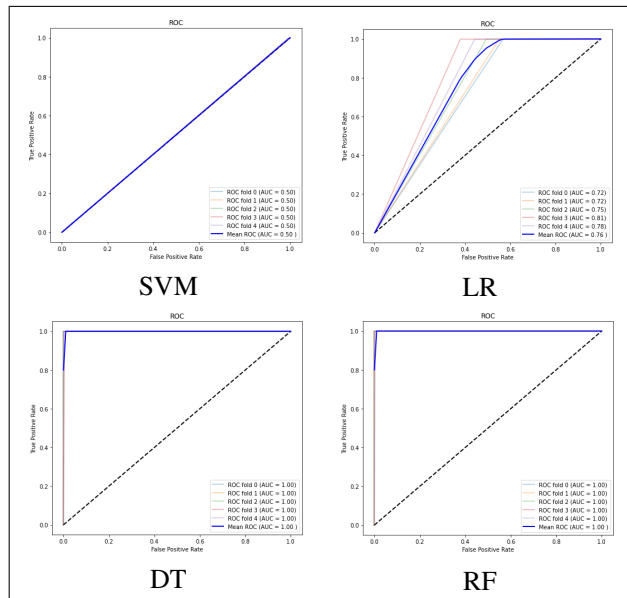
Figure 14. ROC Curve for dataset-3(without Feature Reduction)
